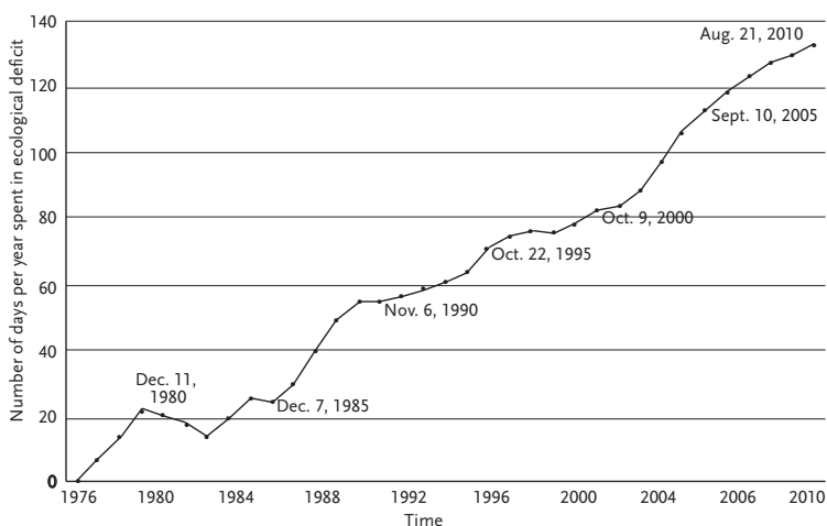
Figuur 3: Earth Overshoot day over time Bron: footprintnetwork.org
